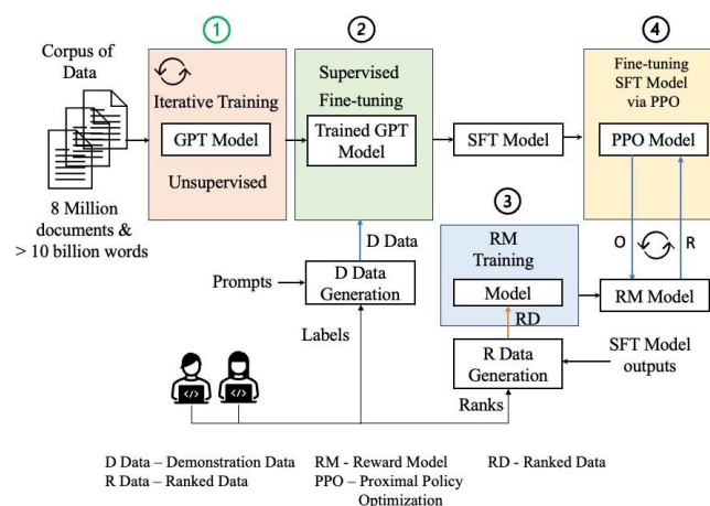
Figure 5. Training chatGPT model.
