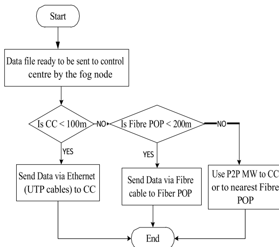
Figure 9: Communication technology choice based on control center and Fibre points of presence locations.
