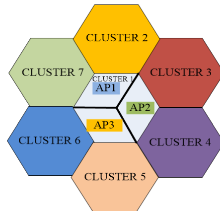
Figure 10: Access network coverage area based on cellular design.
