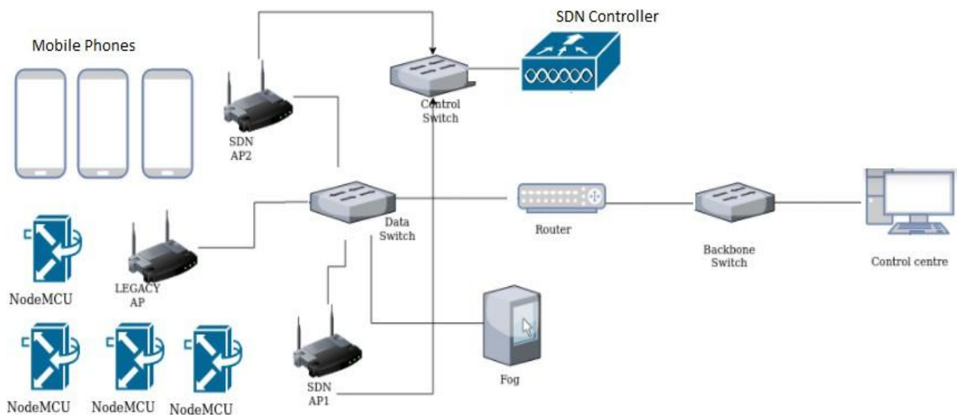
Figure 12. Lab architecture design.
