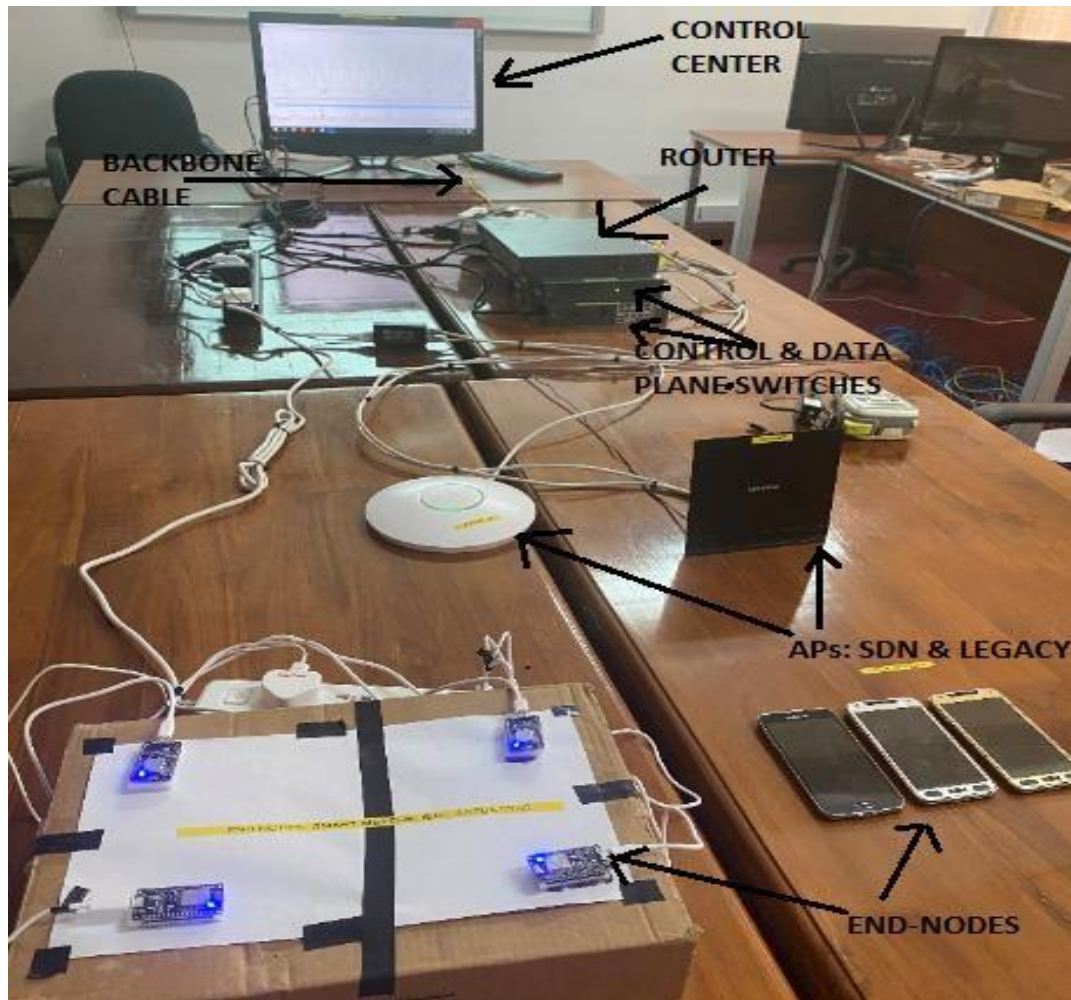
Figure 13. Actual Lab deployment of a hybrid architecture based on hierarchical computing.
