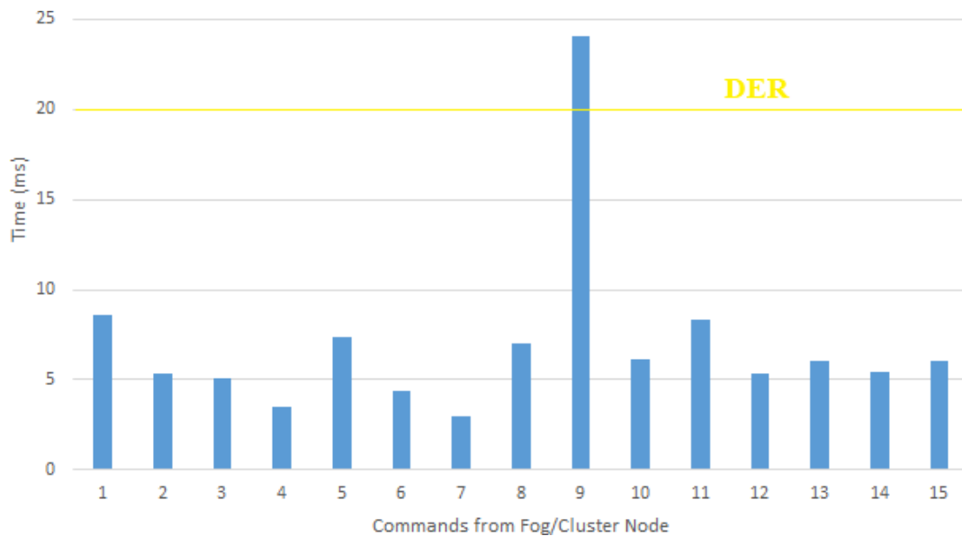
Figure 17. Latency values for Fog/Cluster node commands to End Nodes.
