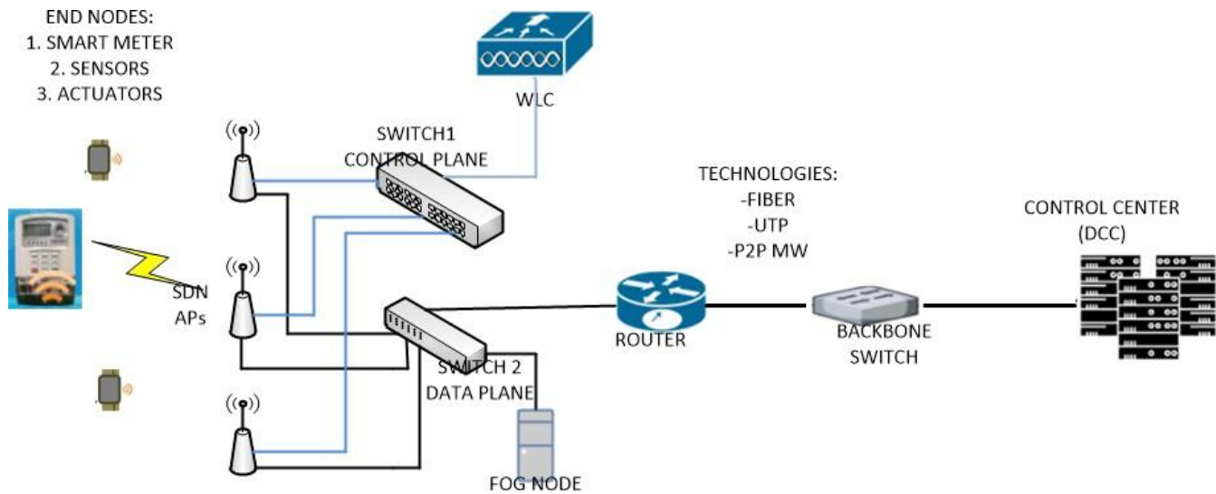
Figure 11. SDN based access network.
