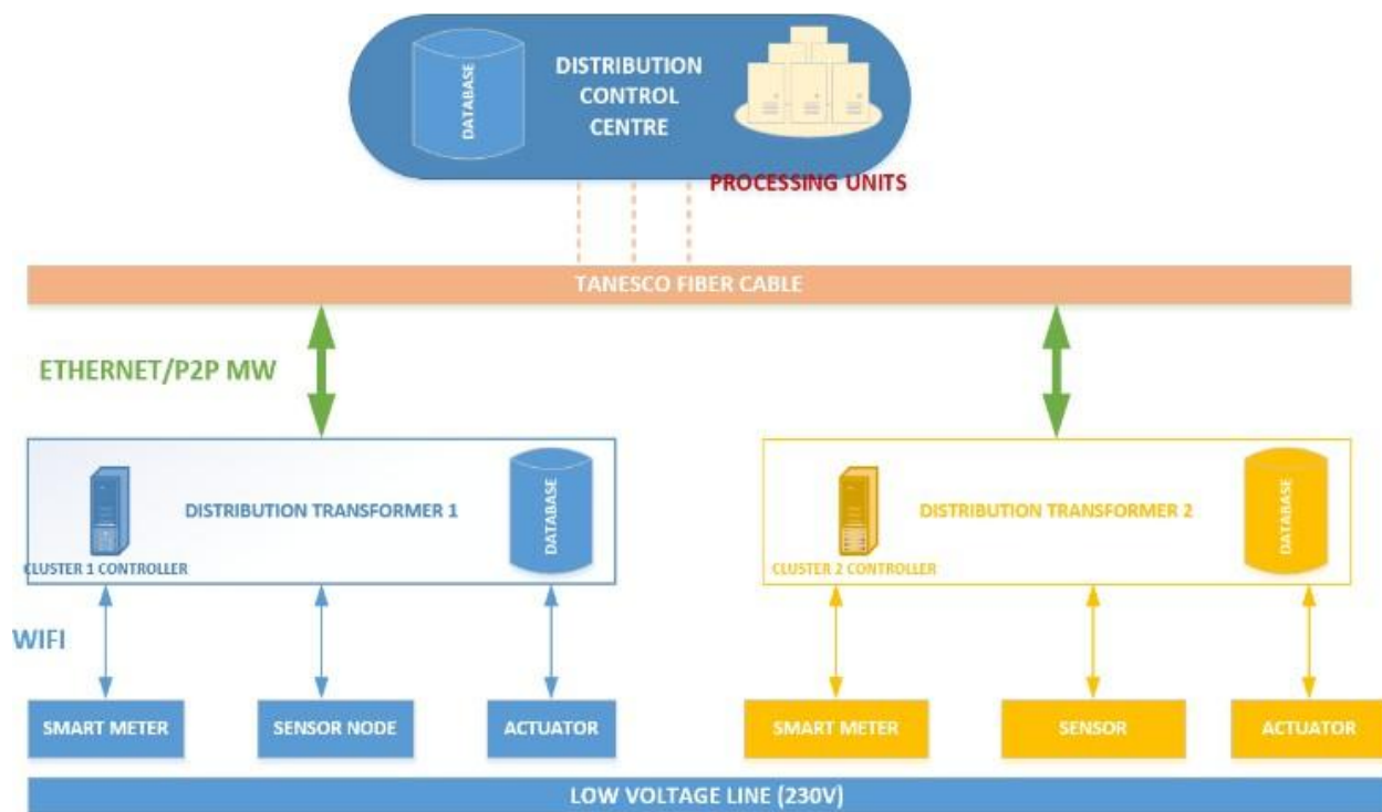
Figure 8: Hybrid communication technologies deployed in the architecture.
