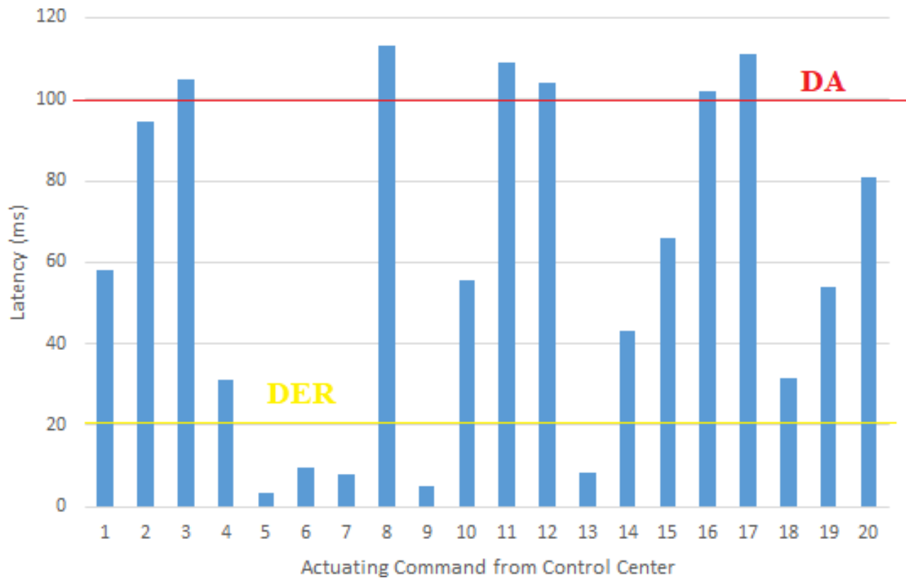
Figure 19. Latency values for CC commands straight to end nodes (centralized approach).
