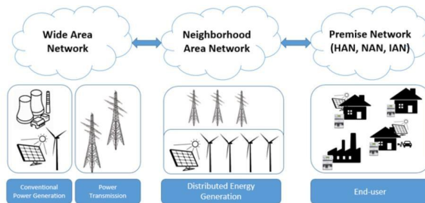
Figure 2. Communication networks in SG [12].
