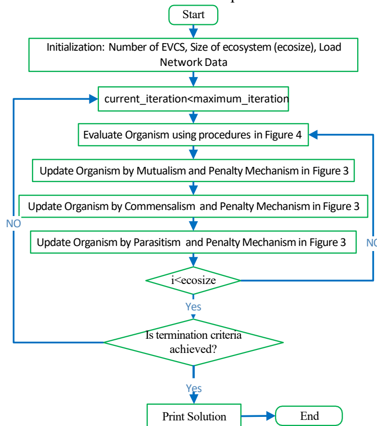
Figure 5. The Proposed SOS with penalty mechanism for placement of EVCS in electrical distribution networks.
