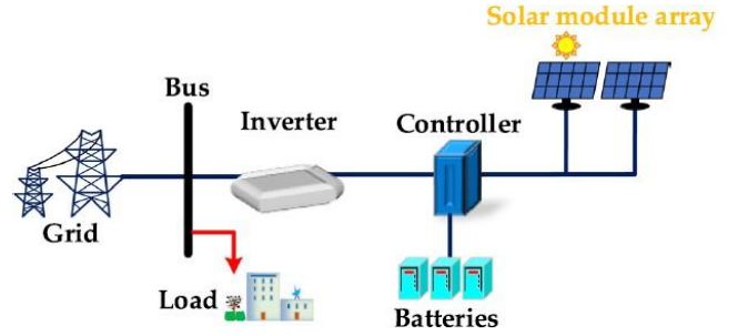
Figure 2. Schematic diagram of grid-connected solar PV [40].
