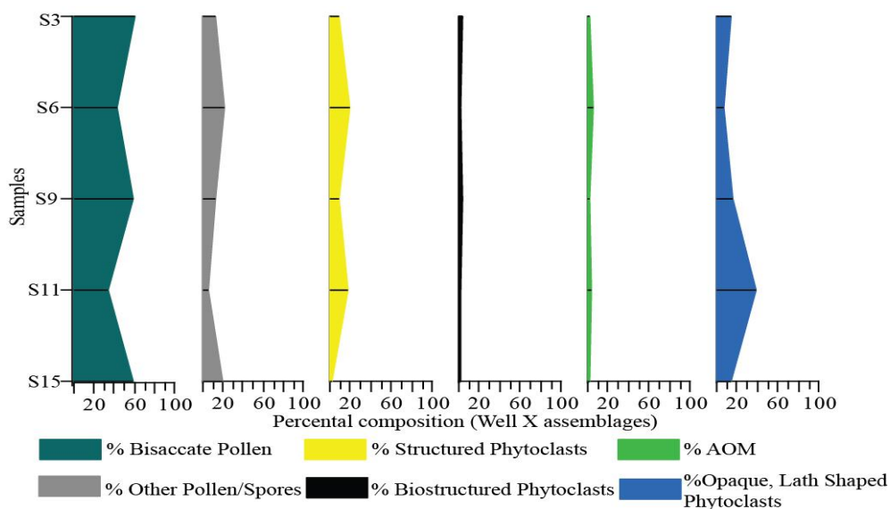
Figure 5: Percentage composition of Well X assemblages.
